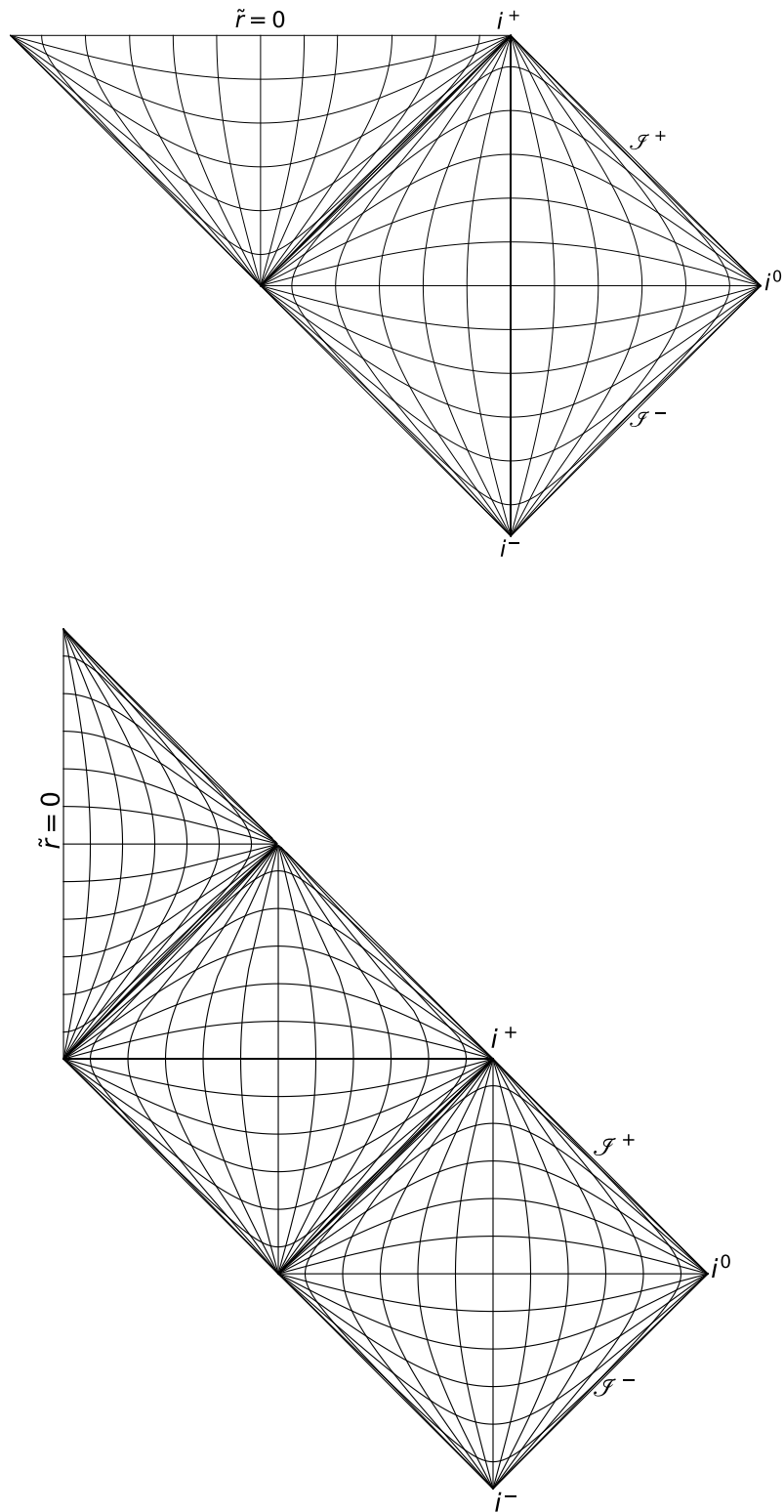
Figure C.1: Schwarzschild and Reissner-Nördstrom Penrose diagrams with lines of constant \tilde{r} and constant \tilde{t} .
