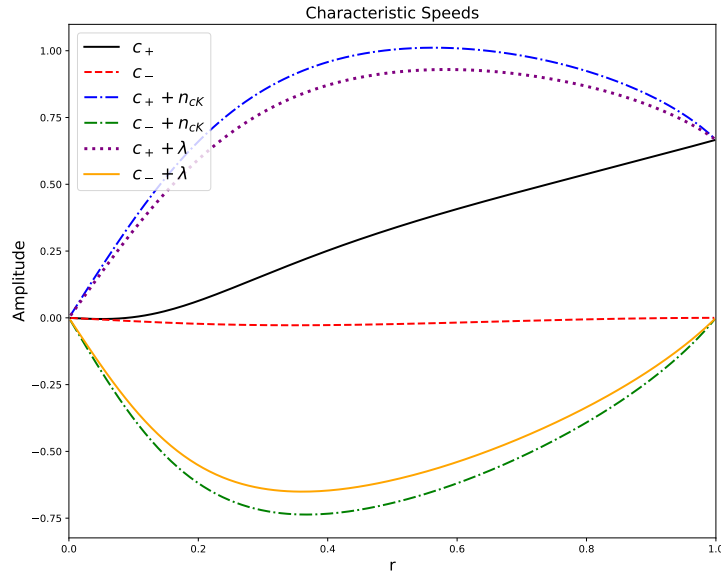
Figure 6.18: Characteristics of the system we are modeling. \lambda is set to 0.8 and n_{cK} to 1.0.
