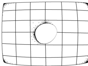
Figure D.1: Region of spacetime with a hole in it. Source: [89].
