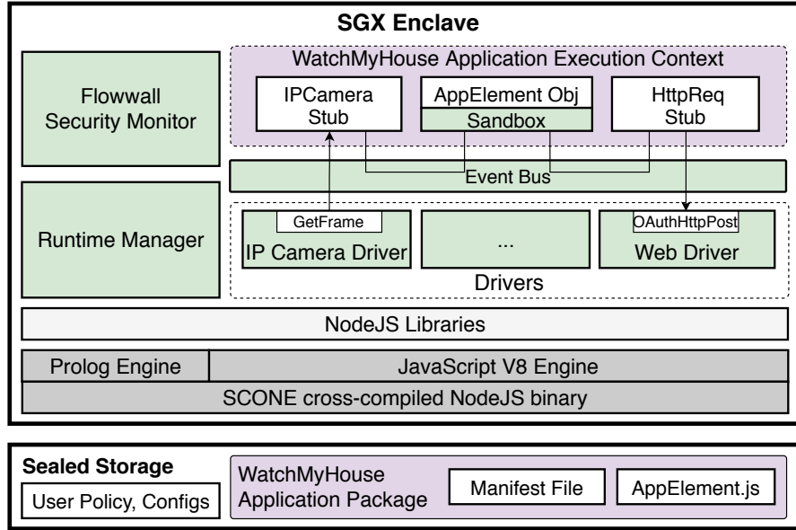
Figure 4.3 – Components of PatIoT TSAR.
