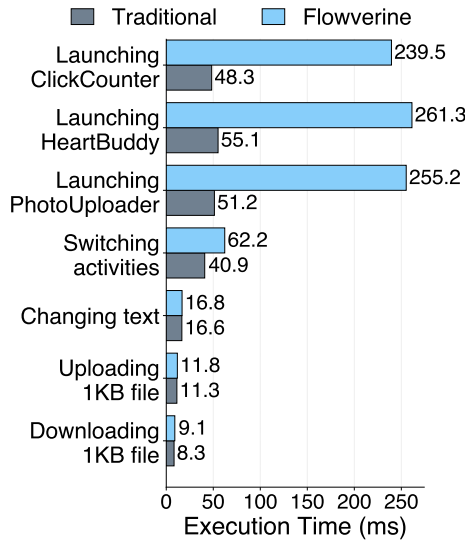
Figure 5.7 – Runtime benchmarking tests results.
