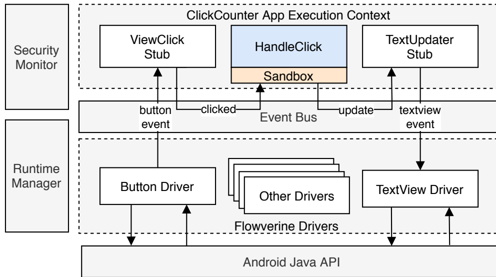
Figure 5.4 – Execution runtime of a ClickCounter application.
