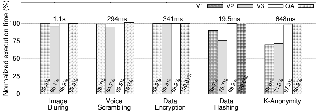
Figure 6.3 – Strict modules performance
