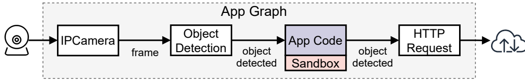
Figure 2.3 – Flow graph of SecurityAlert app.
