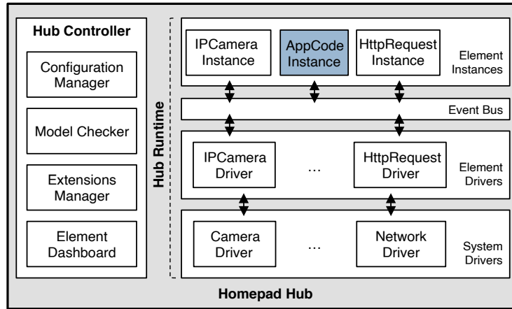
Figure 3.2 – HomePad hub architecture.
