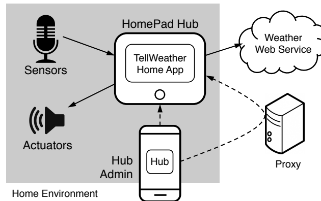
Figure 3.1 – HomePad deployment.
