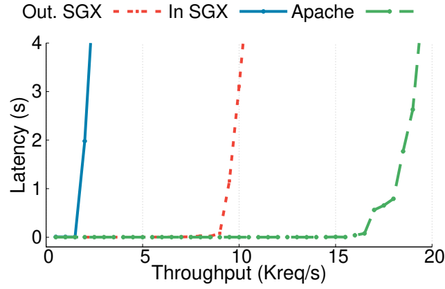
Figure 4.10 – Throughput versus latency evaluation.
