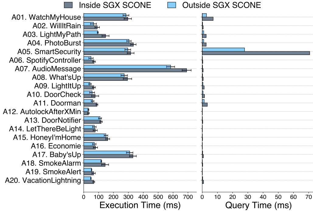
Figure 4.11 – PatrIoT app benchmark performance.
