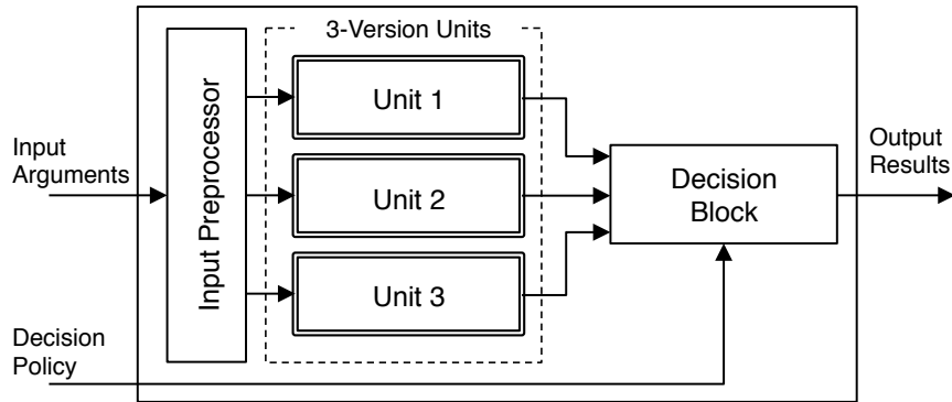
Figure 6.1 – N-version trusted element module (with N=3 ).
