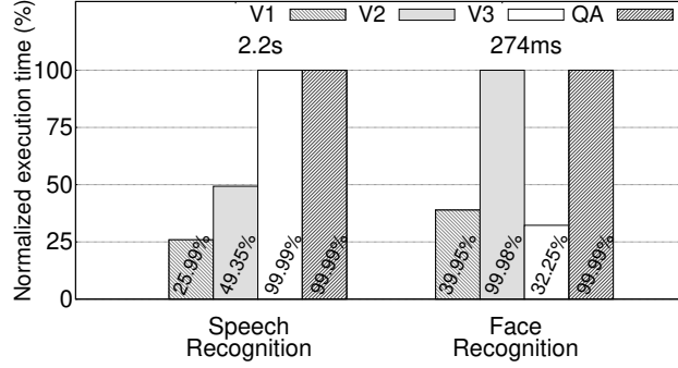
Figure 6.4 – Loose modules performance
