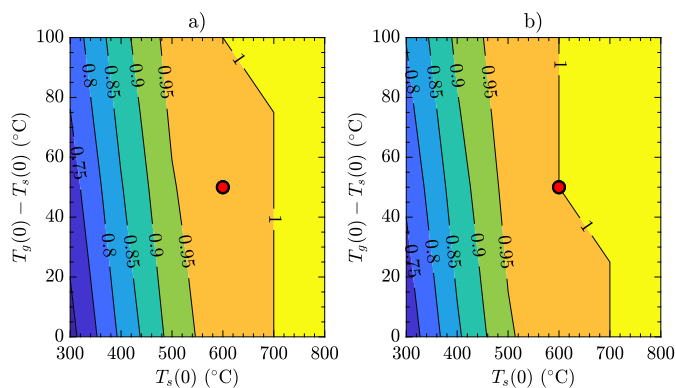
Fig. 21. Molar calcination conversion at reactor heights of (a) 4 m and (b) 6 m as a function of the inlet gas and solids temperatures for the case of imposed irradiance without wall conduction in the angular direction. The nominal operating conditions are indicated by a red circle with a black edge. (For interpretation of the references to color in this figure legend, the reader is referred to the web version of this article.)
