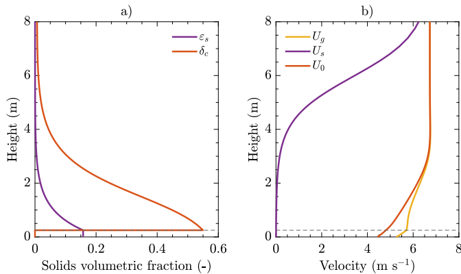
Fig. 13. (a) Solids volumetric fraction and fraction of the wall covered by clusters and (b) gas and solids velocities as a function of the calciner height for the case of imposed irradiance with wall conduction in the angular direction.
