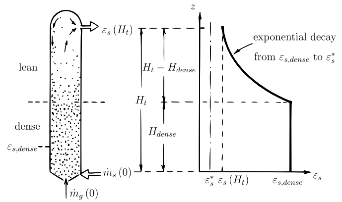
Fig. 2. Variation of the solids volumetric fraction with the reactor height, which gives an insight into the fluid dynamics described by the K-L model.
