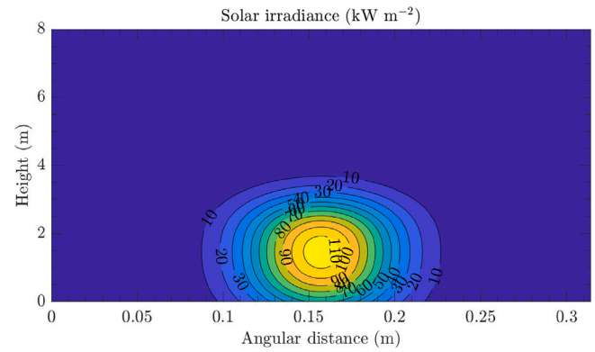
Fig. 5. Concentrated solar irradiance as a function of the calciner height and angular distance.
