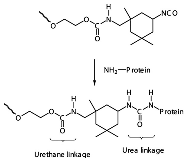
Fig. 2. Reaction between a prepolymer and the amino groups of a protein resulting in a urea linkage [189]. Copyright 2008, Springer. Reproduced with Permission.
