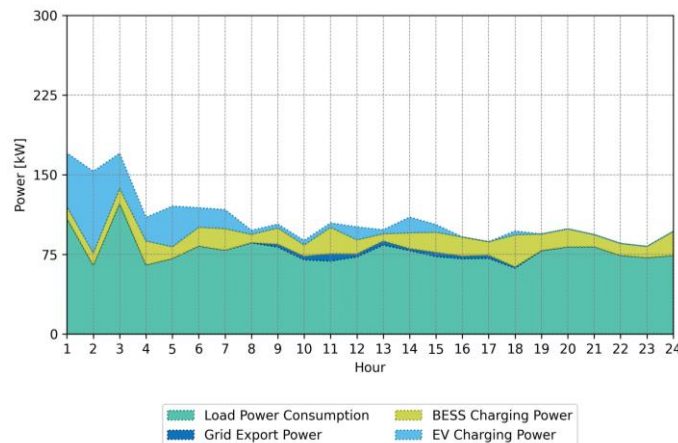
Figure 17 – Net consumption results for metaheuristic model (DO), Method 3
