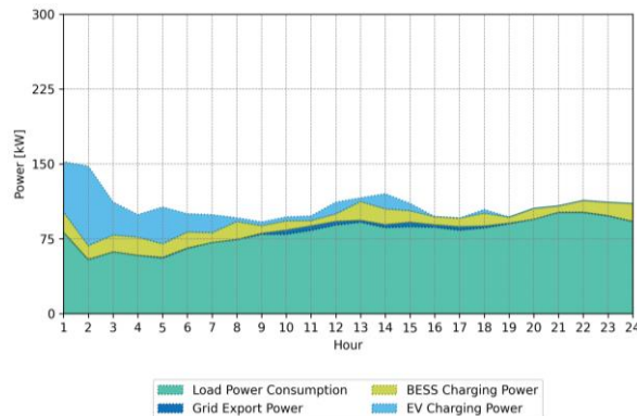
Figure 13 – Net consumption results for metaheuristic model (DO) Method 1
