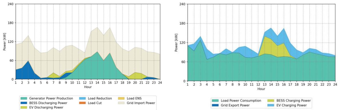
Figure 9 – Production (left side) and Consumption (right side) results for deterministic model, Method 2
