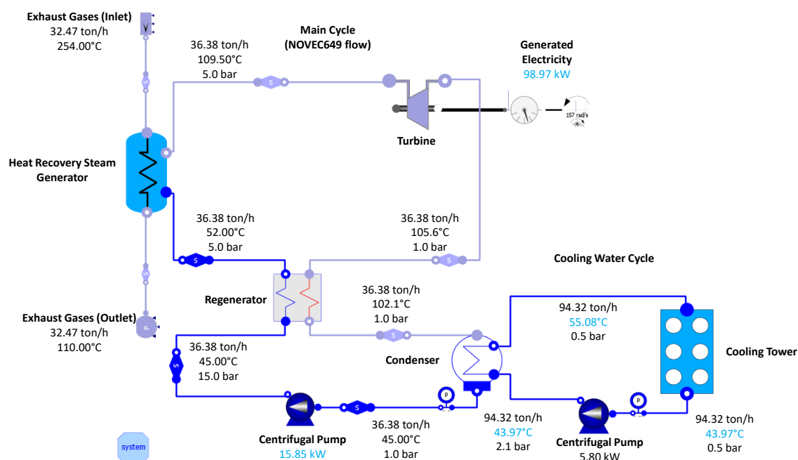
Figure 3.10. Test model for the validation of the Organic Rankine Cycle (ORC) system model (to-be-validated key variables are signalized in a lighter colour)
