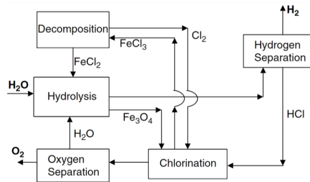
Figure 2.12. Flowsheet representations for thermochemical water splitting systems: a) Metal oxide cycle, b) Sulphur-iodine cycle, c) Iron-chlorine cycle (adapted from [307], [319] and [322])
