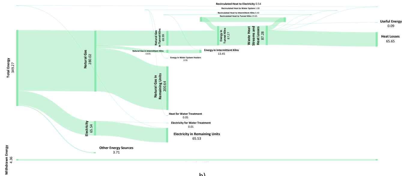
Figure 6.3. Sankey Diagram for the Plant Energy Balance in Case-study 2: a) Baseline Scenario, b) Improved Scenario (Energy consumption unit of TJ/year)
