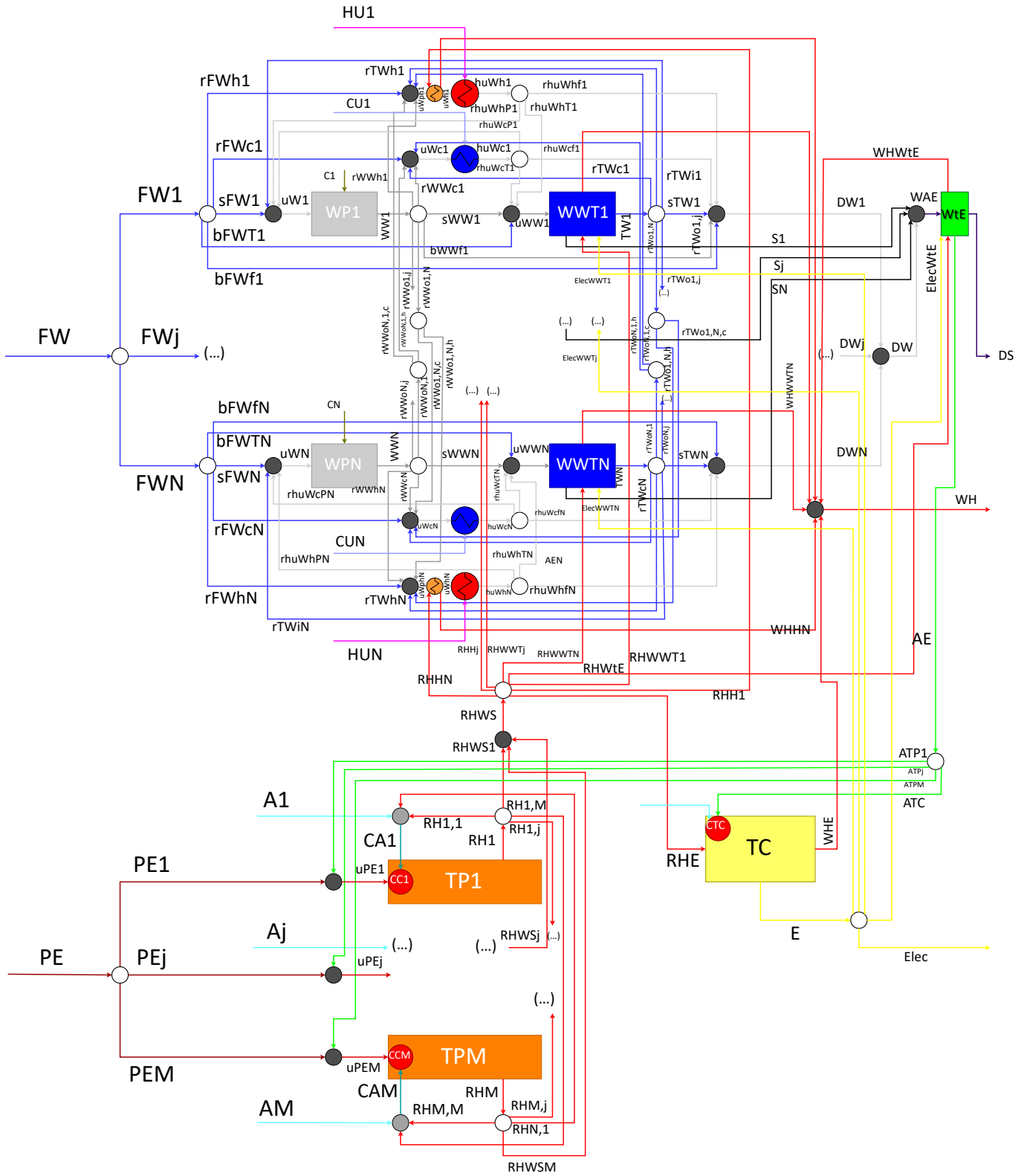
Figure 3.7. Generalized superstructure for WEIS Configuration 1 (Standard)
