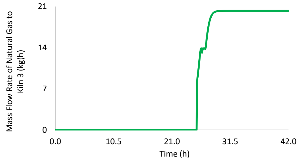
Figure 5.6. Optimisation results along time for the mass flow rate of natural gas of a) Kiln 1, b) Kiln 2, c) Kiln 3 and d) Kiln 4
