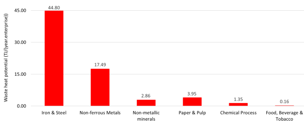
Figure 2.17. Waste heat potential levels for several industrial sectors in the European Union (data gathered from [21,363–366])
