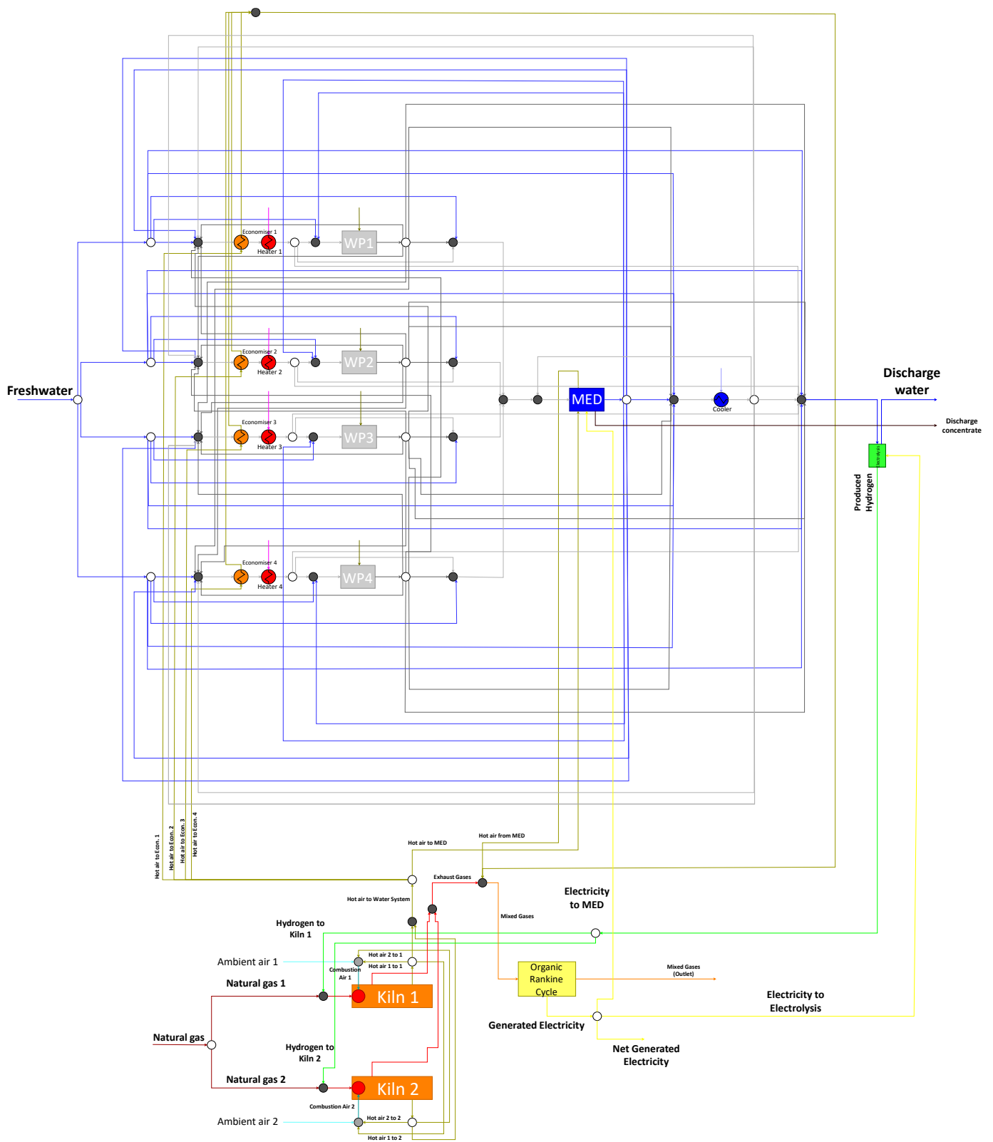
Figure 4.3. Flowsheet assembling of Scenario 1
