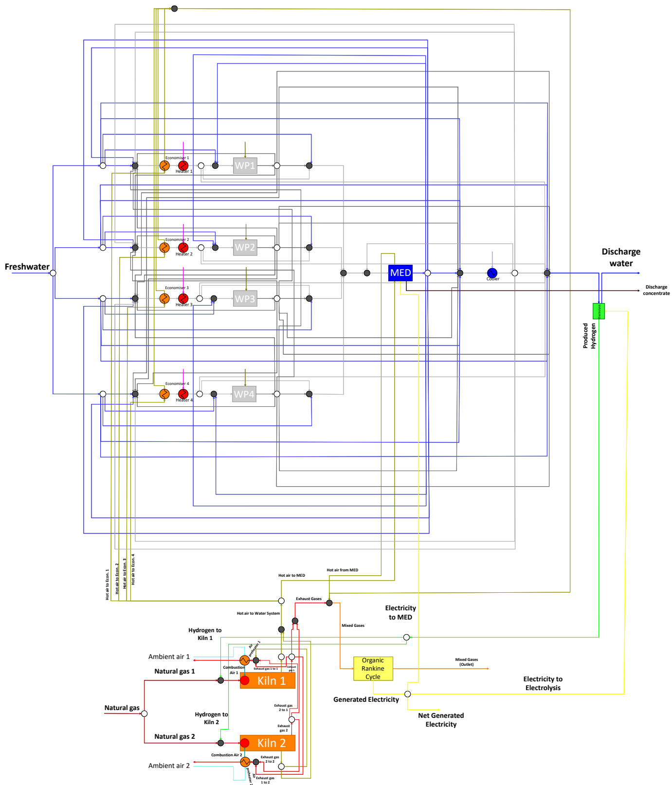
Figure 4.4. Flowsheet assembling of Scenario 2
