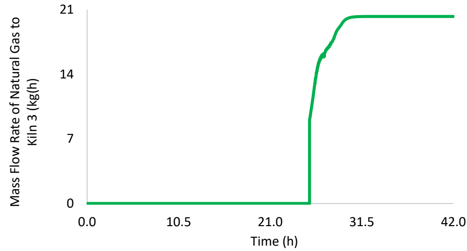
Figure 5.15. Final optimisation along time for the mass flow rate of natural gas of a) Kiln 1, b) Kiln 2, c) Kiln 3 and d) Kiln 4
