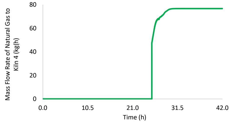
Figure 5.15. Final optimisation along time for the mass flow rate of natural gas of a) Kiln 1, b) Kiln 2, c) Kiln 3 and d) Kiln 4
