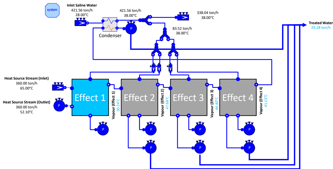
Figure 3.13. Test model for the validation of the Multi-effect distillation (MED) system model (to-be-validated key parameters are signaled in a lighter colour)
