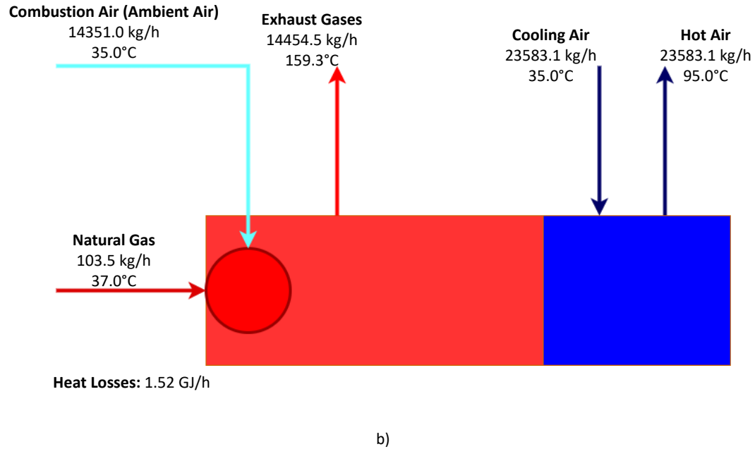
Figure 4.2. Flowsheets of Tunnel Kilns including stream data (mass flow rate and temperatures) and heat losses (Case-study 1): a) Tunnel Kiln 1, b) Tunnel Kiln 2
