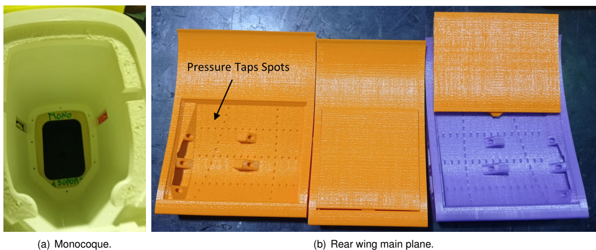
Figure 4.6: Hollow components.
