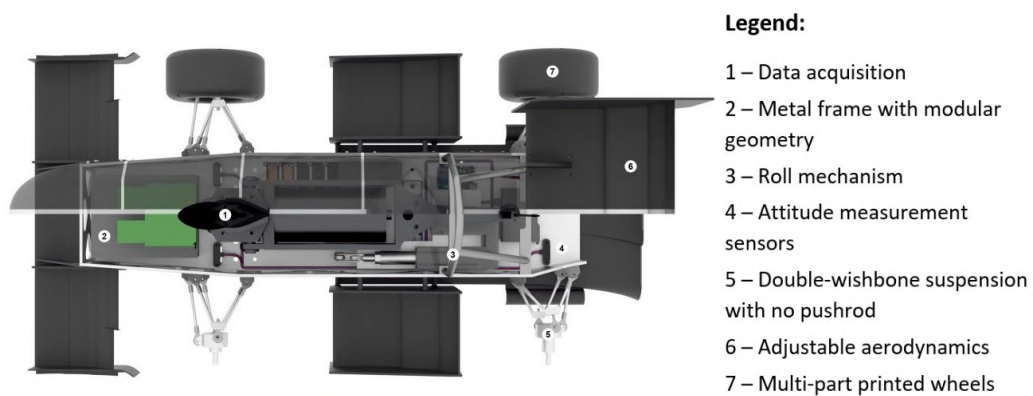
Figure 1.9: SSUFS wind tunnel model scheme. From [7].
