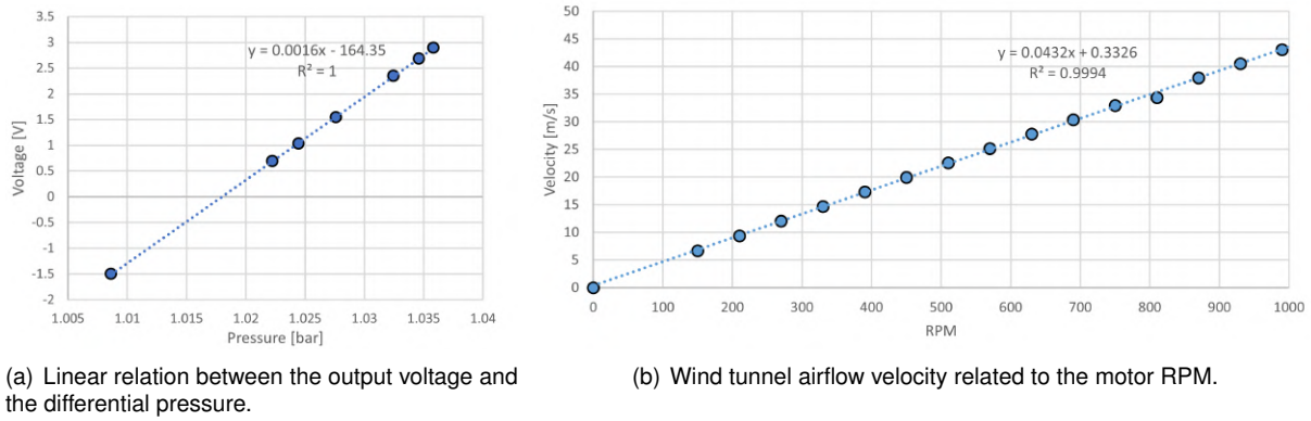
Figure 2.22: Wind tunnel apparatus calibration.
