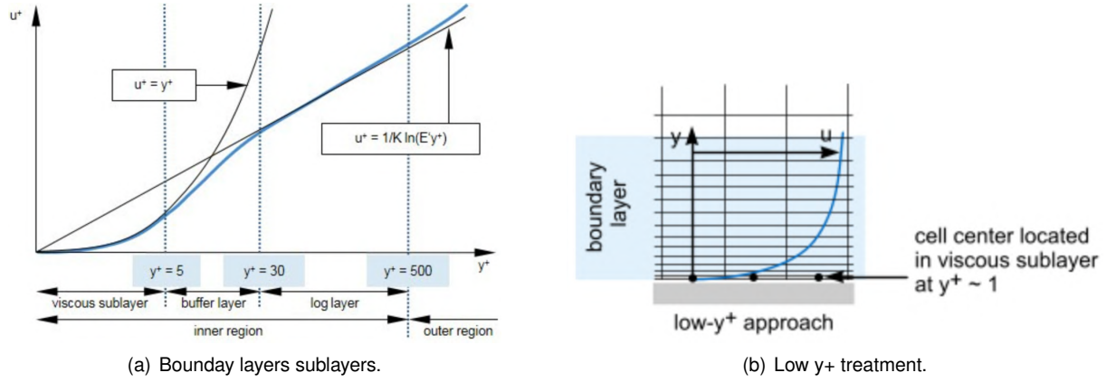
Figure 3.11: Boundary layer treatment.
