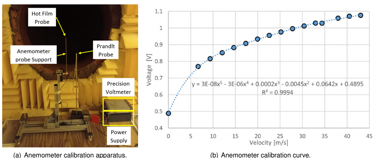
Figure 2.23: Anemometer calibration.
