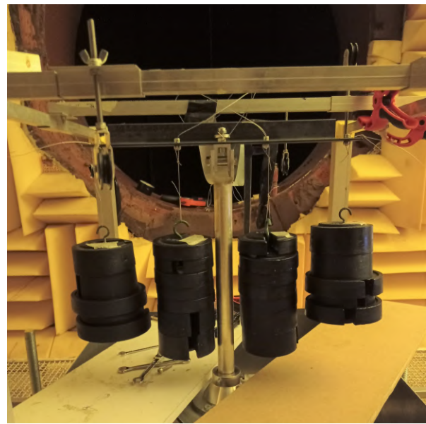
(b) F_z load case, around 36 N in negative z direction. Load is applied symmetrical to eliminate any moments.
