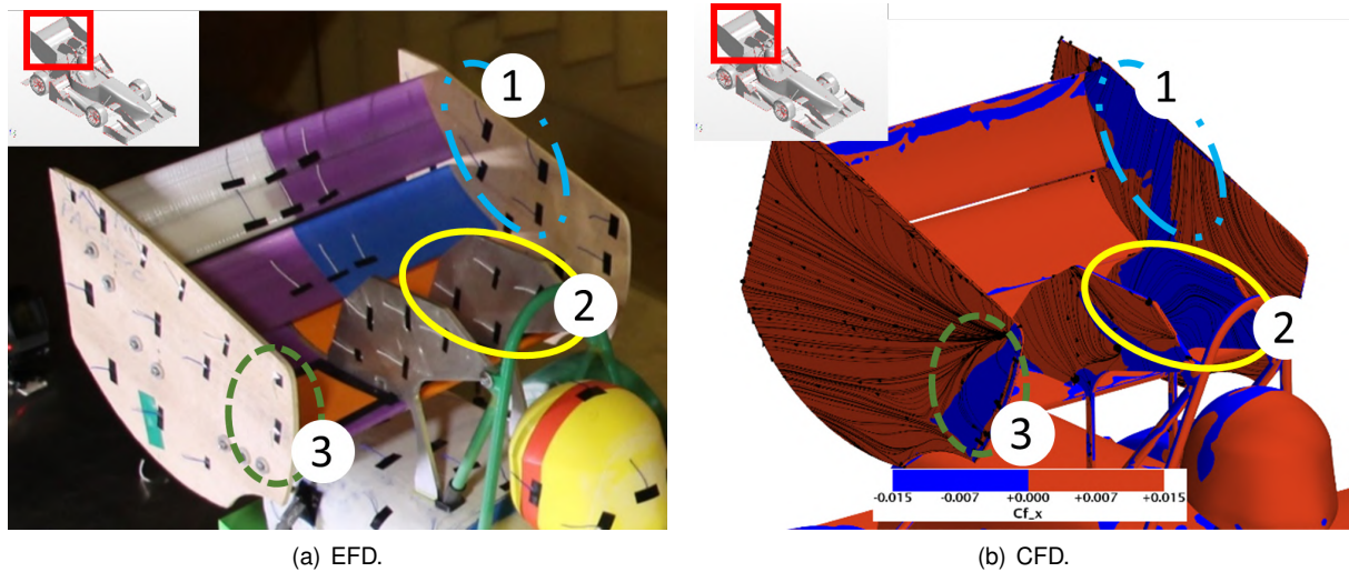
Figure 5.9: Rear wing flow visualization ( RH1 ).
