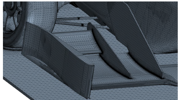
(b) Front Wing and Wheel
