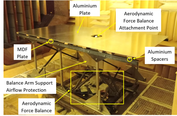
(b) Ground installed.
