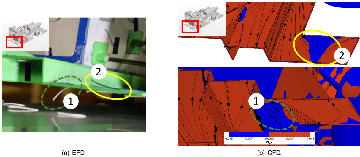
Figure 5.13: Diffuser flow visualization ( RH1 ).
