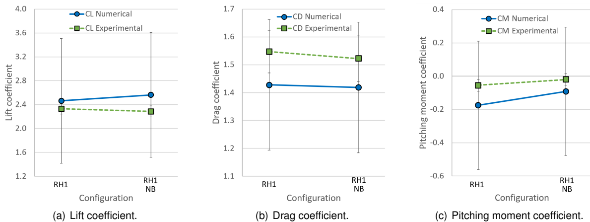
Figure 5.16: Bullhorn study aerodynamic loads.
