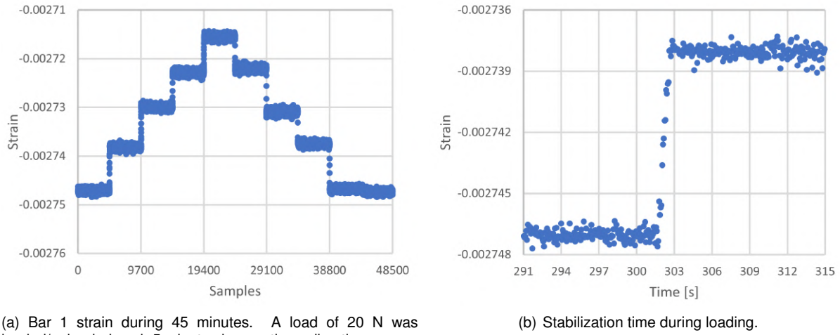
Figure 2.11: Force balance stabilization.
