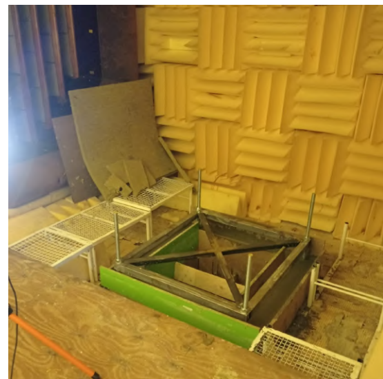
(b) Frame structure installation.
