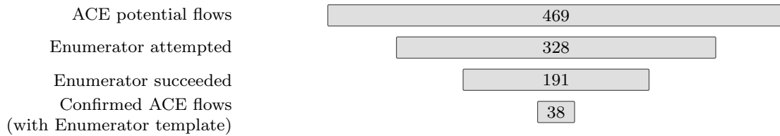
Figure 4.7: How many flows were processed by the Enumerator and how many were successfully exploited. We consider that Enumerator is successfull when it provides a correct completion to the given prefix.
