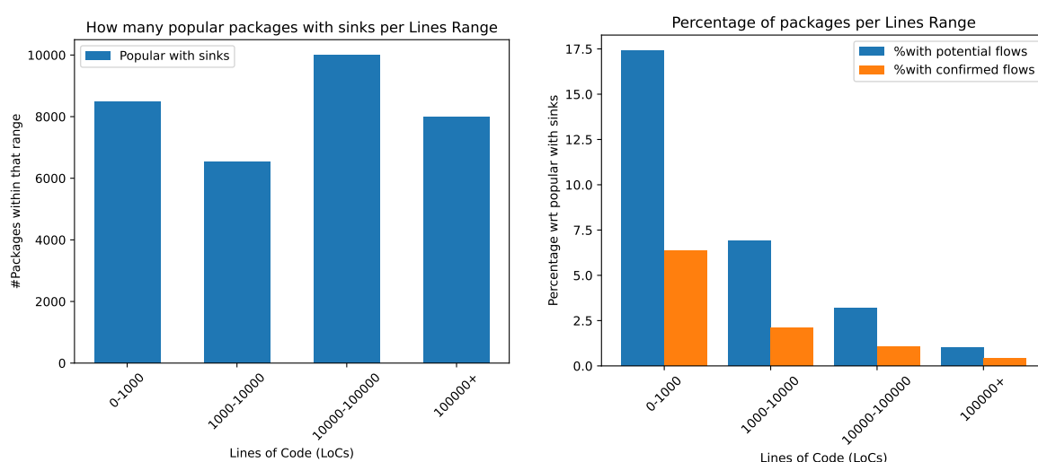
Figure 7.4: Frequency of packages within ranges of lines of code counts, split into "with sinks", "with potential flows" and with "confirmed flows".
