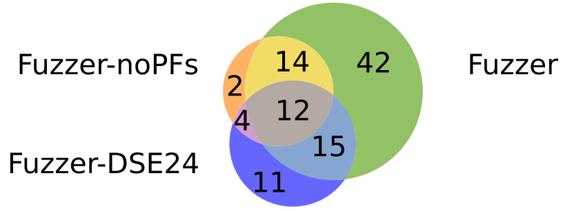
Figure 3.13: Comparison of confirmed flows found across Fuzzer, Fuzzer-noPFs and Fuzzer-DSE24 (RQ2a).
