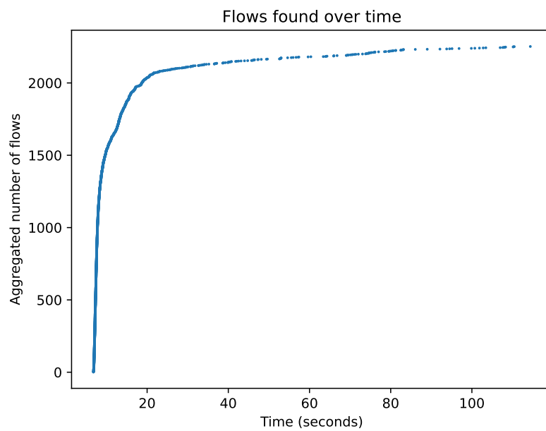
Figure 7.8: Number of flows discovered (y-axis) when we vary the fuzzing timeout.
