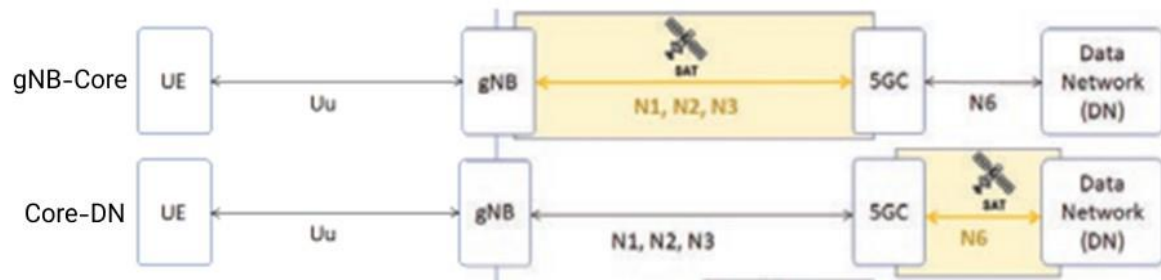
Figure 2-17 Possible Scenarios for backhaul access (extracted from [LQRZ23]).
