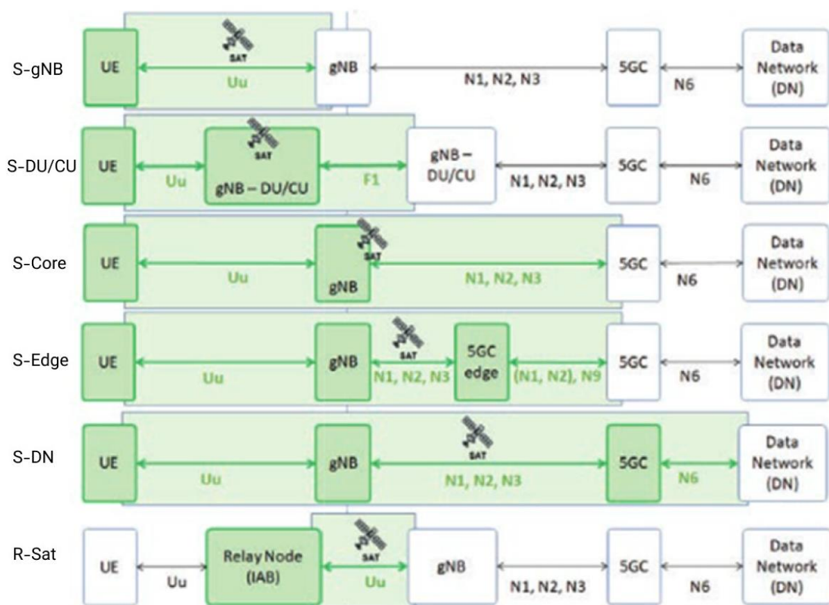
Figure 2-16 Possible Scenarios for direct access (extracted from [LQR23]).
